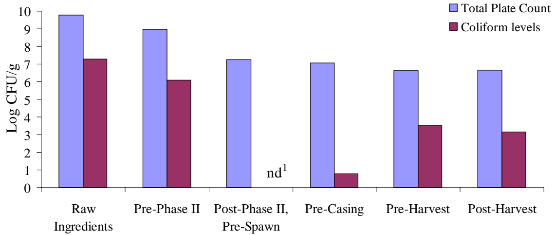
Figure 1. Changes in total aerobic bacteria and coliforms during a complete crop cycle. 1 none detected (<1 CFU/g)
