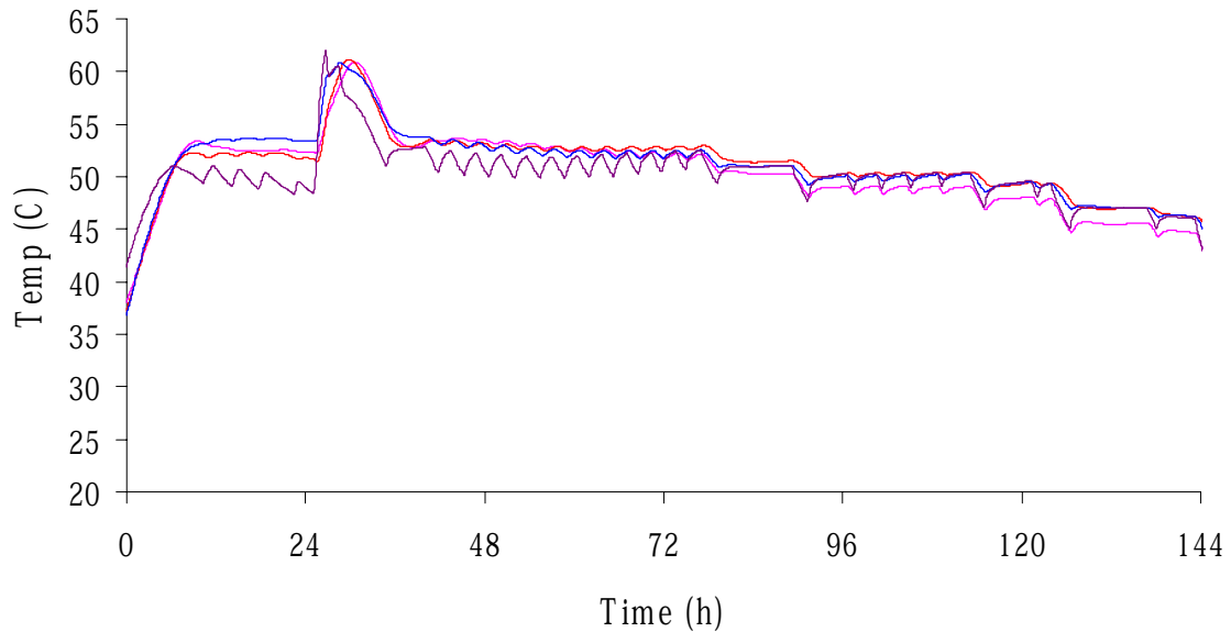
Figure 2. Temperature profile of compost in bags during a standard 6-day Phase II pasteurization and conditioning protocol.
